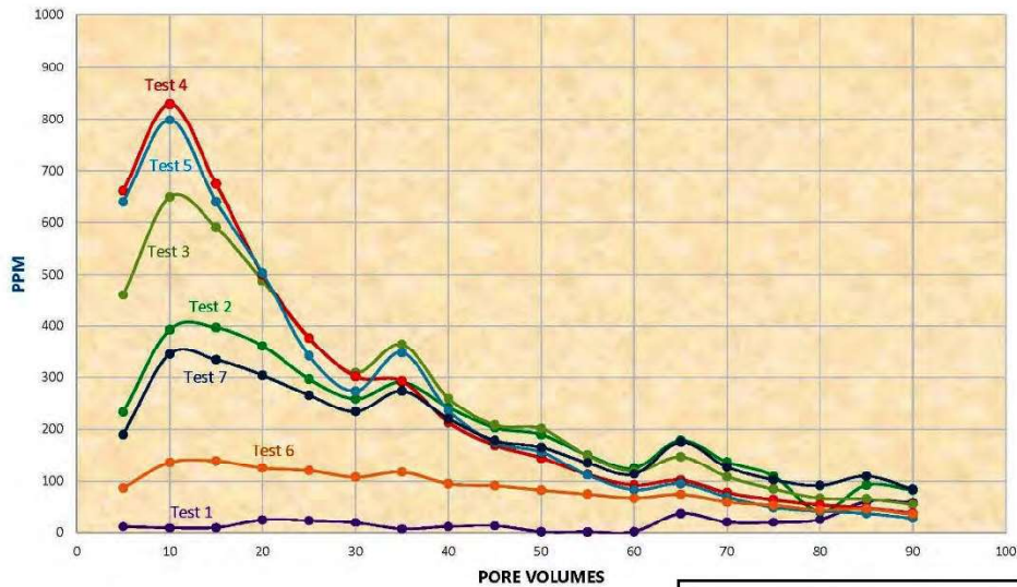
Figure 15 Uranium Recovery Curves Head Grade Comparison
